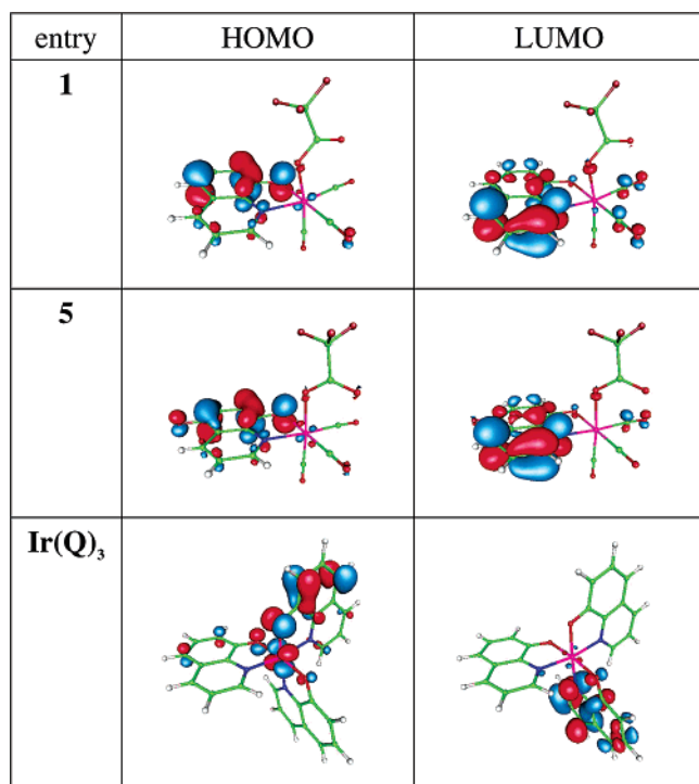
Figure 5. HOMO and LUMO of complexes 1 , 5 , and Ir(Q) 3 . Note that the lowest-lying state in both singlet and triplet manifolds is dominated by the HOMO → LUMO transition. To avoid redundancy, only complexes 1 and 5 are shown for the quinolinolate Os(II) complexes.
